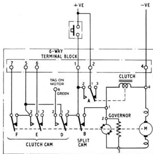
Fig. 2. Circuit diagram
