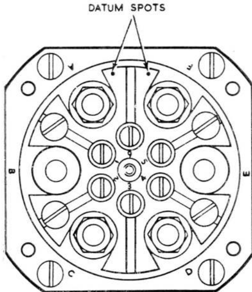
Fig. 4. Terminal arrangement
