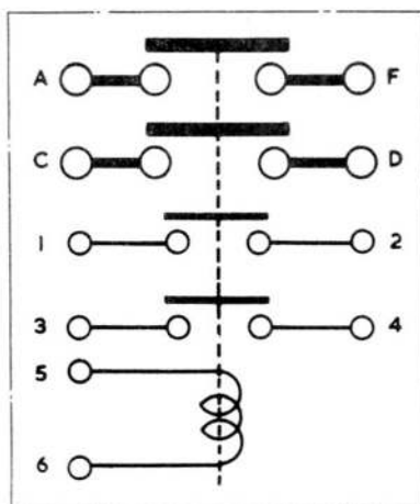
Fig. 3. Circuit diagram
