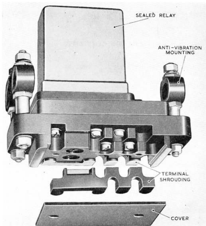
Fig. 1. Magnetic switch, Type 16B, No. 4
