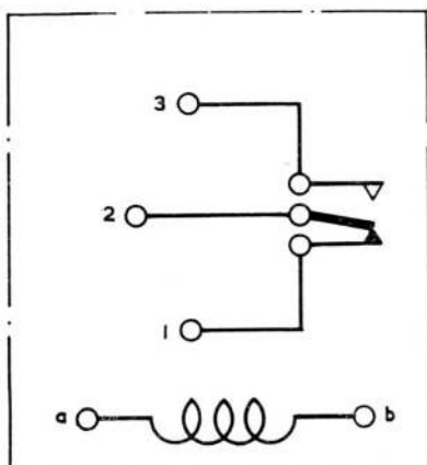
Fig. 2. Circuit diagram
