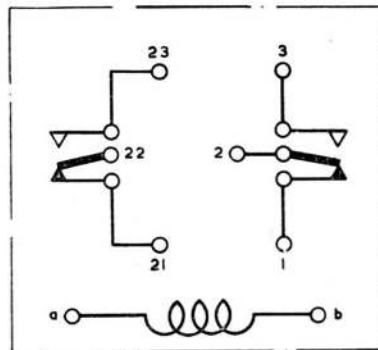
Fig. 2. Circuit diagram
