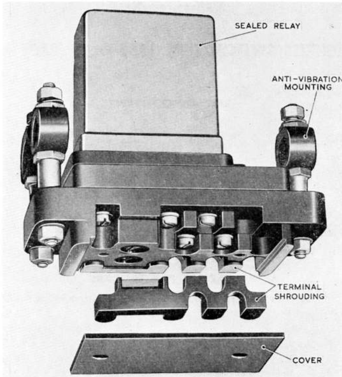
Fig. 1. Magnetic switch, Type 16B, No. 5
