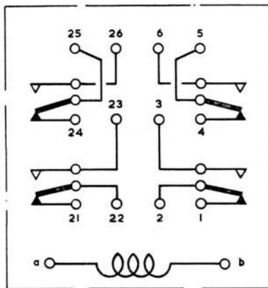
Fig. 2. Circuit diagram
