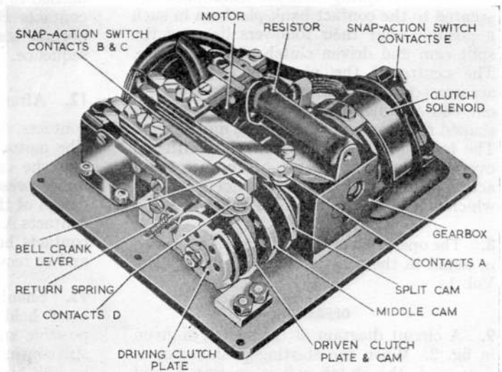
Fig. 1. Time switch, Type FHM/A/24
