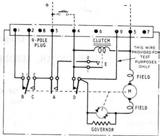
Fig. 2. Circuit diagram
