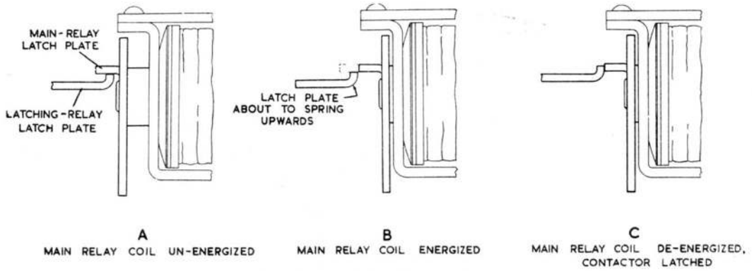
Fig. 3. Details of latching mechanism
