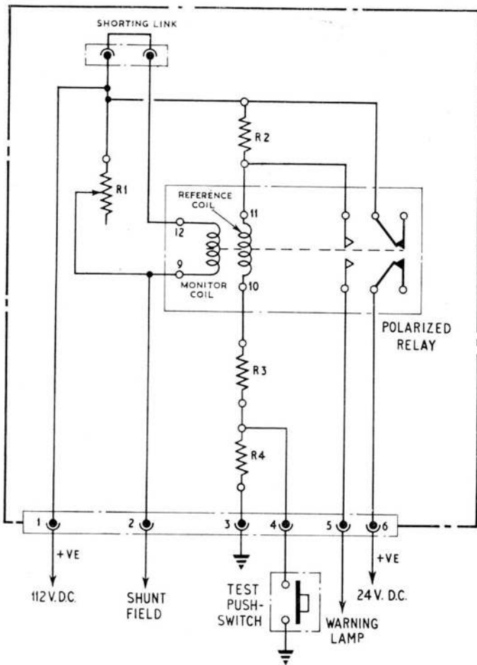
Fig. 2. Circuit diagram
