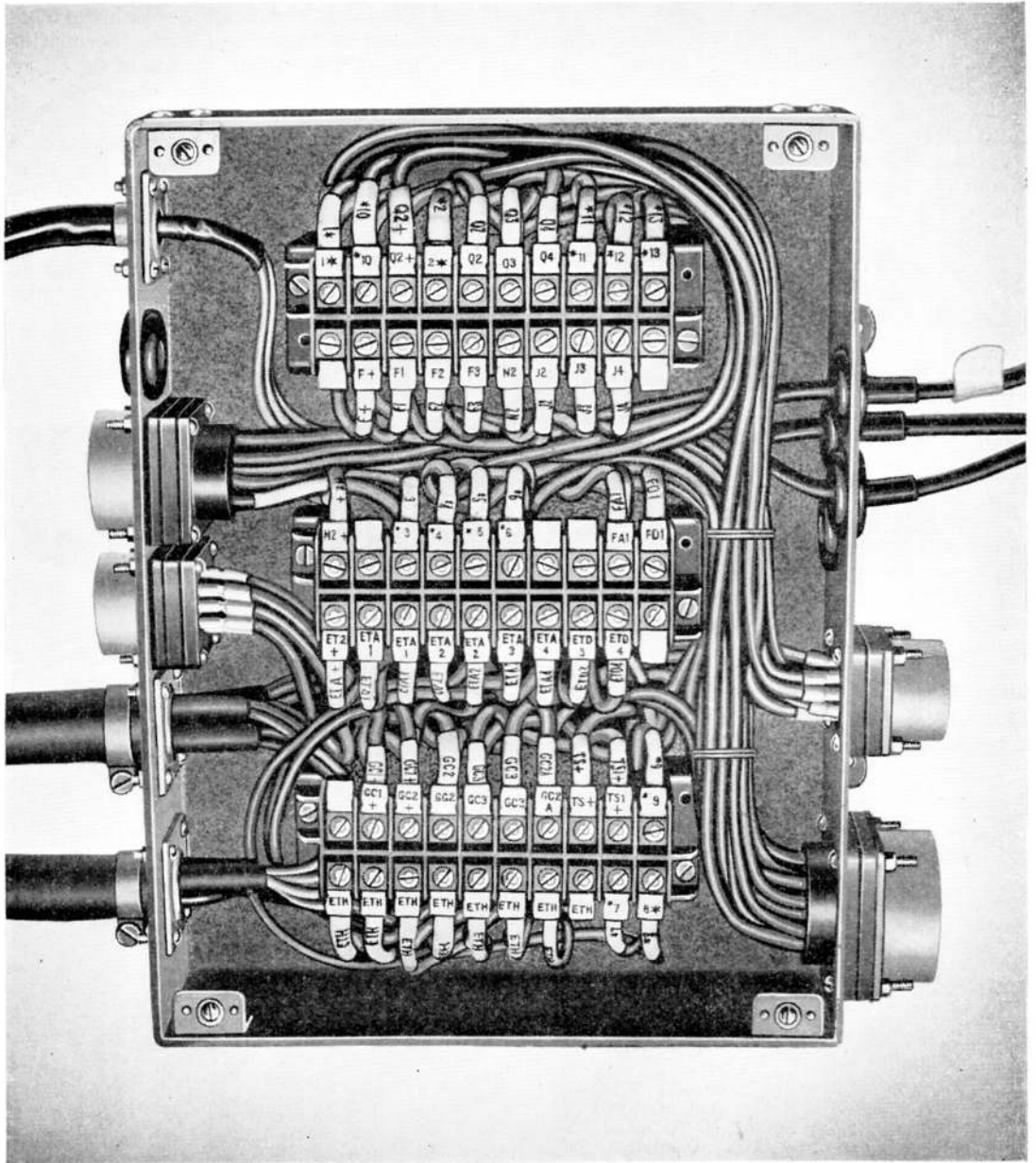
Fig. 13. Typical junction box
