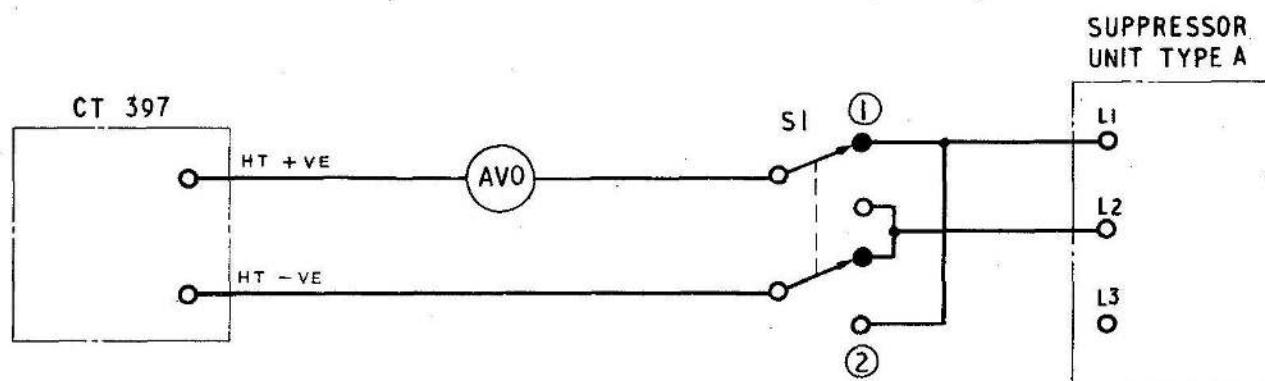
Fig. 1 Test Circuit
