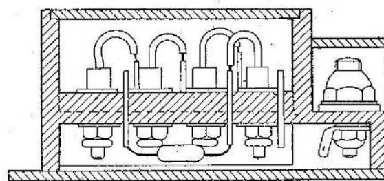
Fig. 2. Internal view
