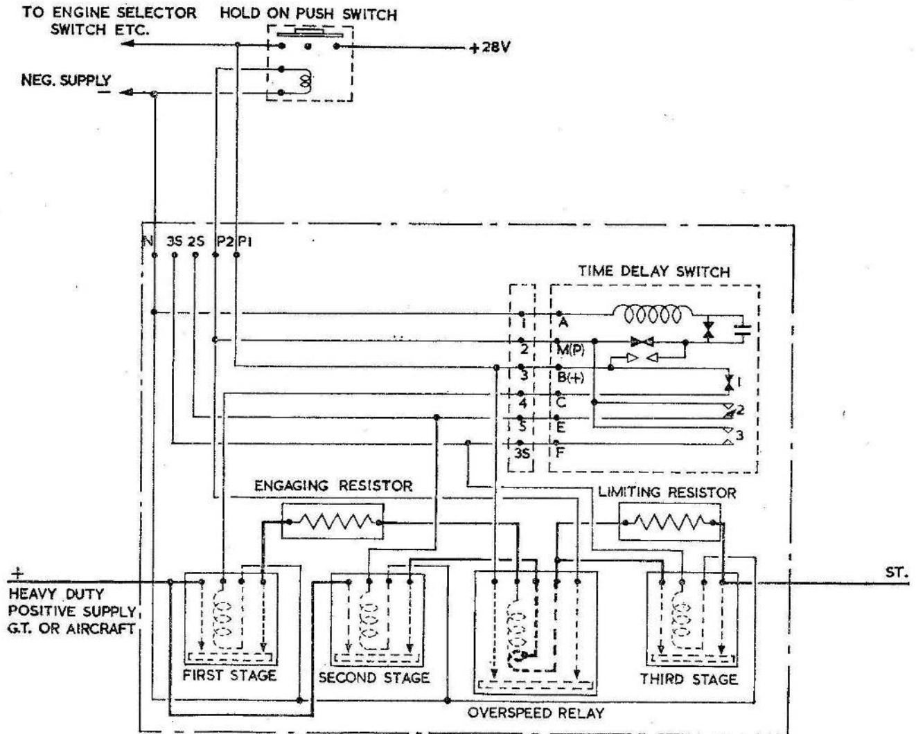
Fig. 2. Diagram of internal connections
