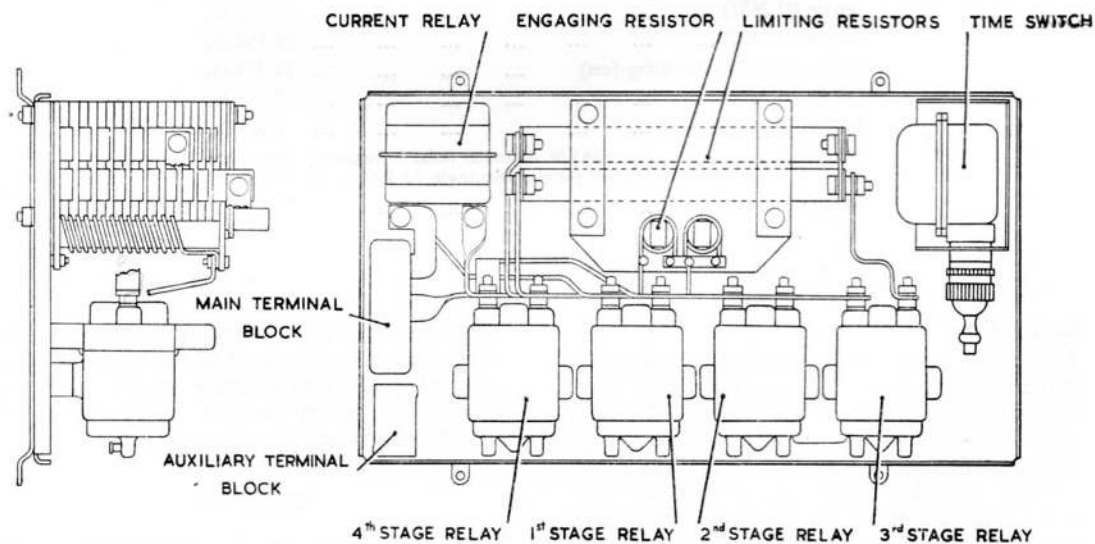
Fig. 2. U2602 starting switch
