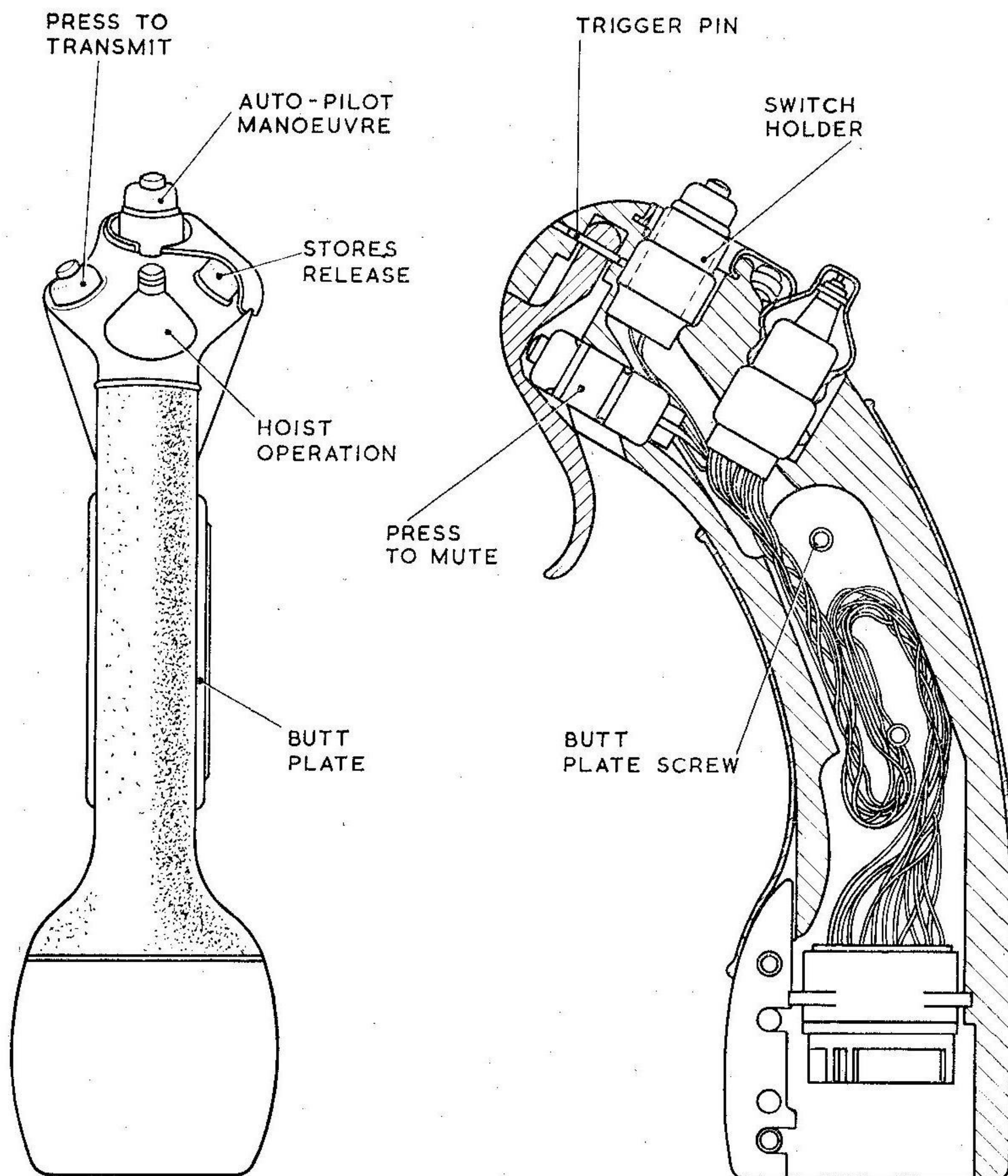
Fig. 1. Typical handle
