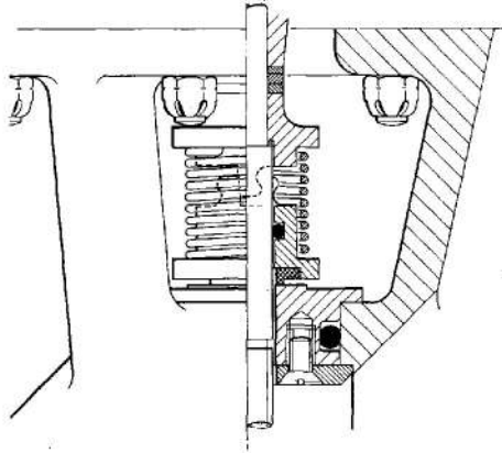
Fig. 1. Dynamic seal arrangement, SPM.7 Mk. 3 pump
