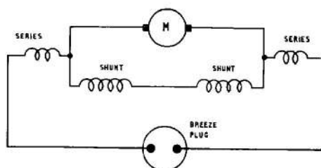
Fig. 1. Circuit diagram—SPM.7 pumps
