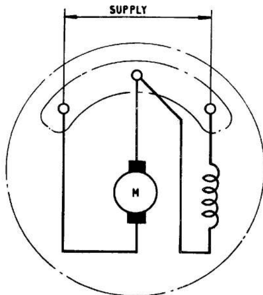
Fig. 3. Circuit diagram
