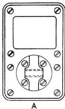
Fig. 1. Alternative positions of rear end fitting on actuators, Types CZ53681/1 and /2
