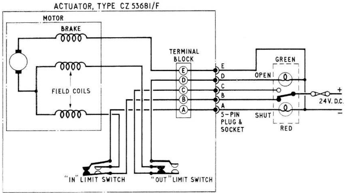
Fig. 8. Wiring diagram of actuator, Type CZ53681/F
