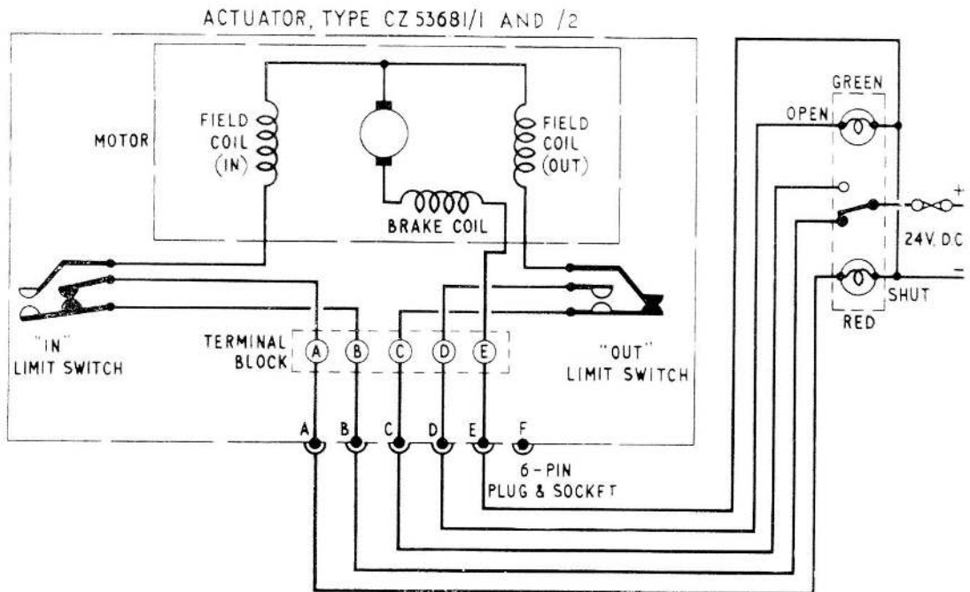
Fig. 7. Wiring diagram of actuators, Types CZ53681/1 and /2
