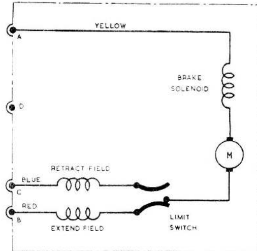
Fig. 1. Circuit diagram, actuator, Type A0215
