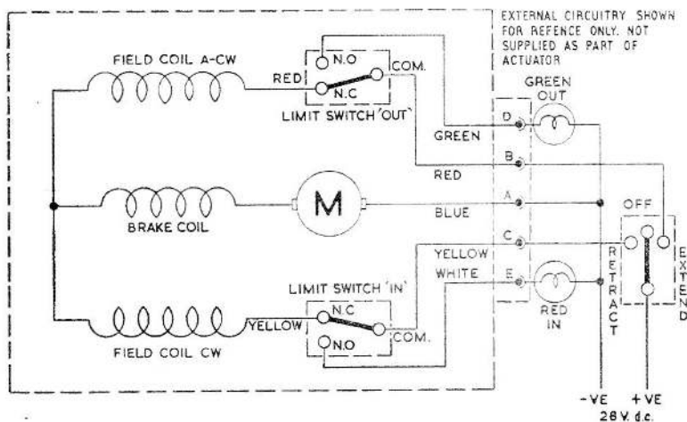
Fig. 3. Circuit diagram
