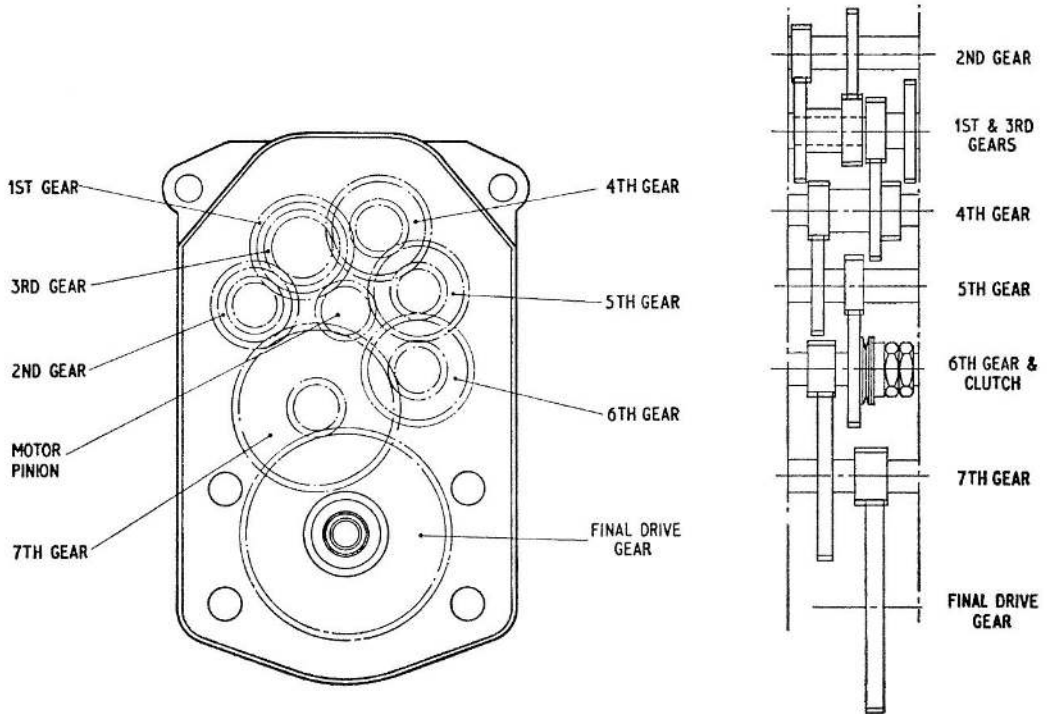
Fig. 2. Arrangement of gearbox
