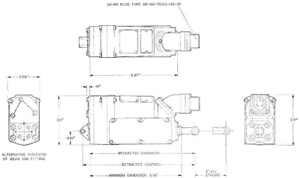
Fig. 6. Installation diagram
