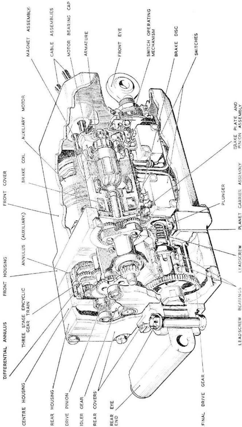
Fig. 1. Cut-away view of simplified Stoat actuator
