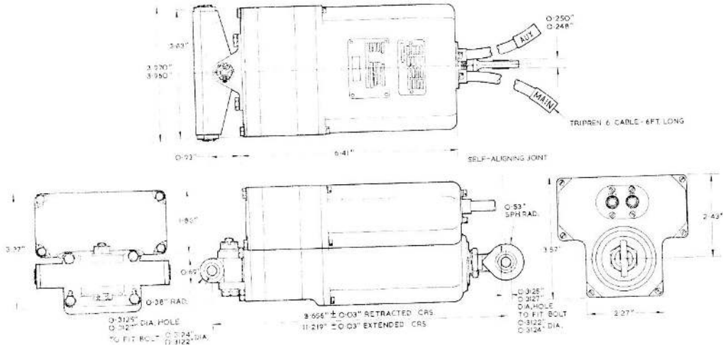
Fig. 1. Installation drawing
