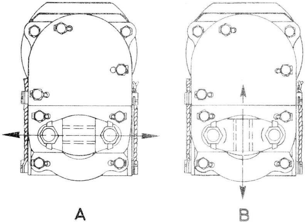
A B Fig. 2. Alternative position of rear end fitting
