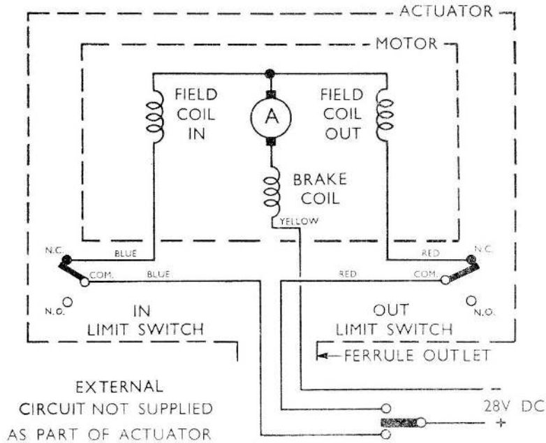
Fig. 3. Circuit diagram
