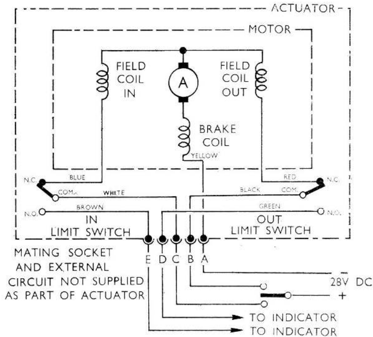
Fig. 4. Typical circuit diagram
