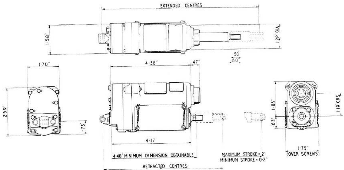
Fig. 2. Installation details
