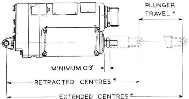
Fig. 2. Installation details
