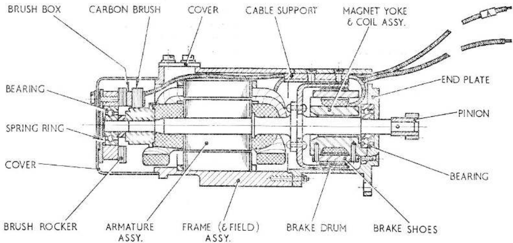
Fig. 2. Section of motor
