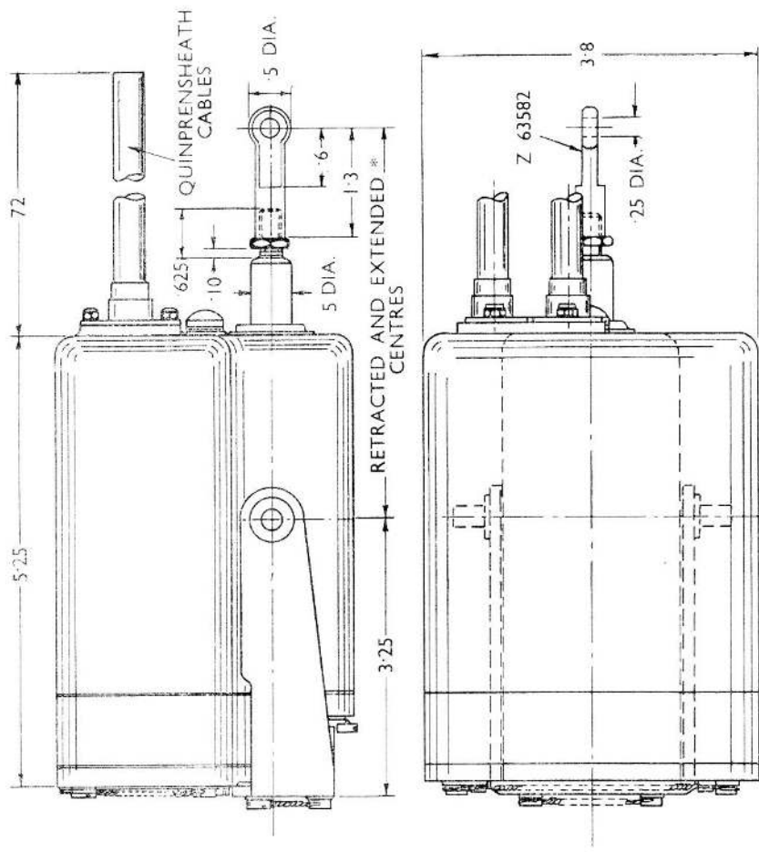
Fig. 1. Installation drawing
