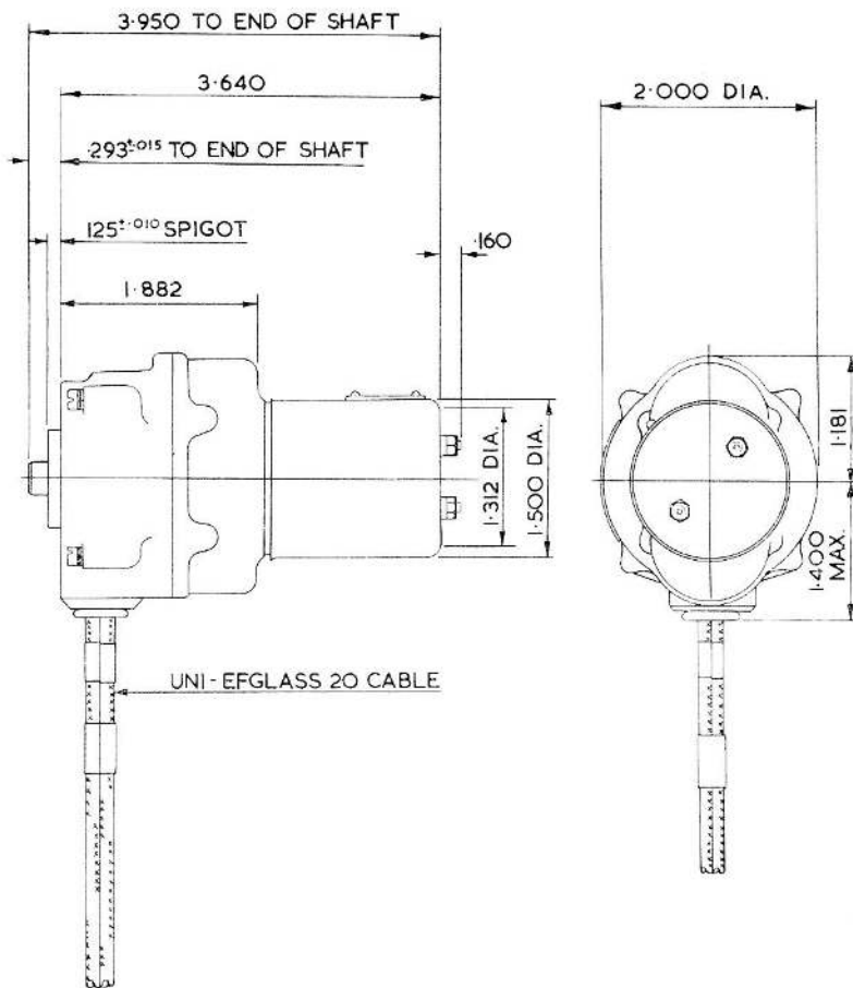
Fig. 2. Installation details
