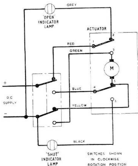
Fig. 1. Circuit diagram
