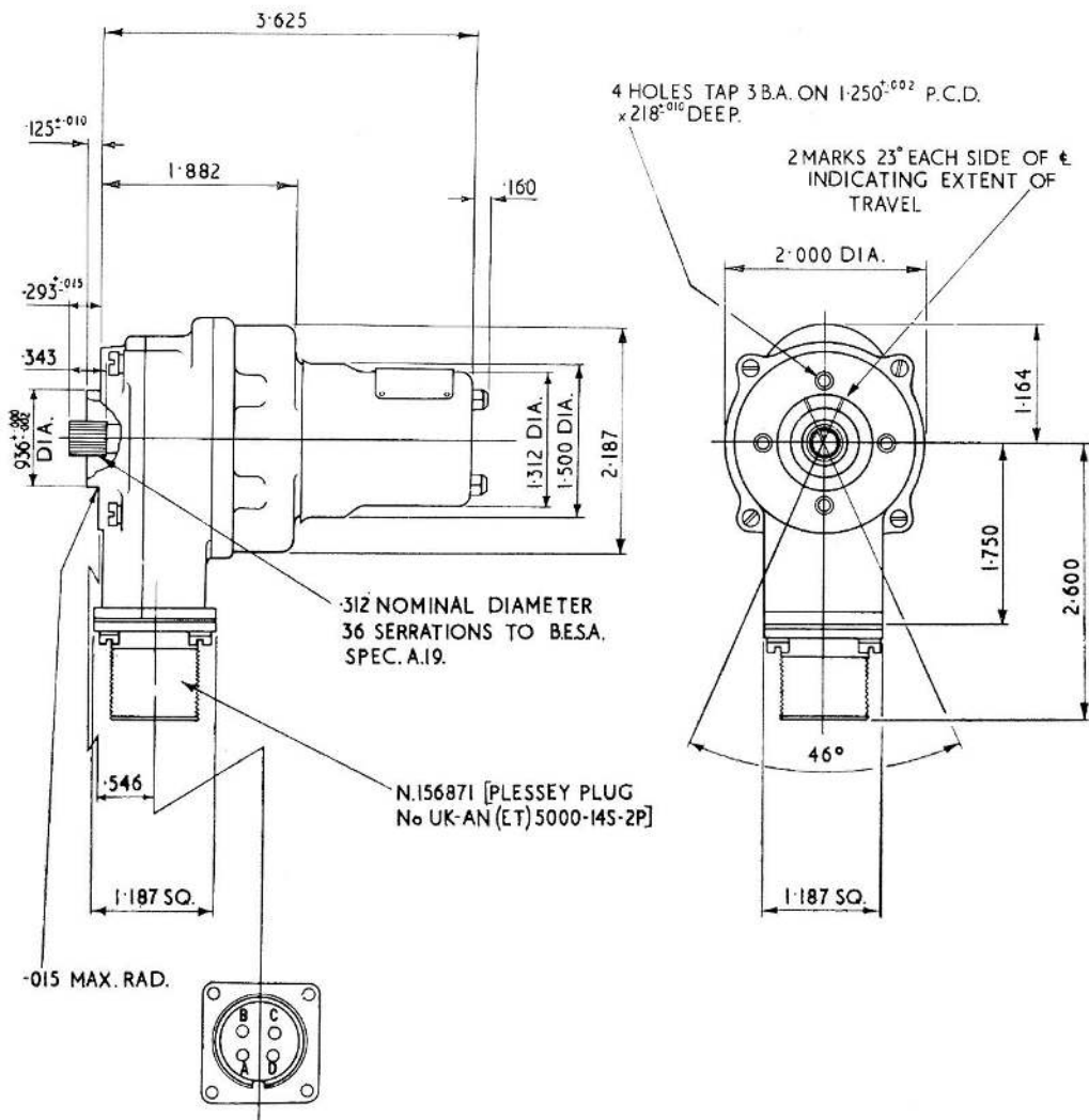
Fig. 2. Installation details
