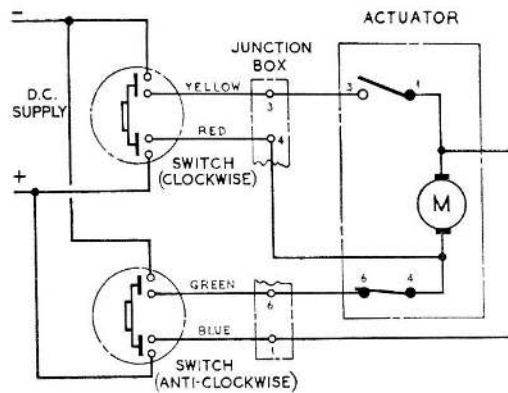
Fig. 2. Circuit diagram
