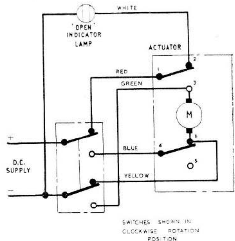
Fig. 1. Circuit diagram
