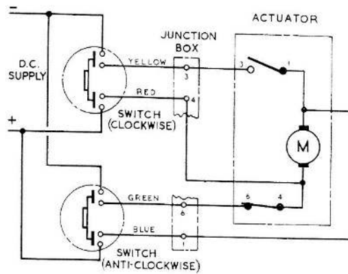
Fig. 2. Circuit diagram
