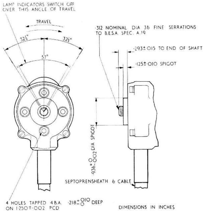
Fig. 2. Installation details
