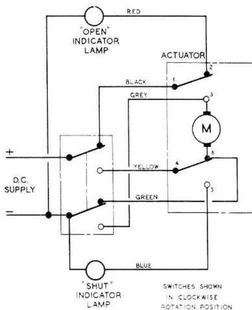
Fig. 2. Circuit diagram
