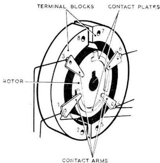
Fig. 2. Arrangement of switch block
