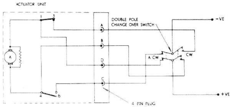
Fig. 1. Circuit diagram
