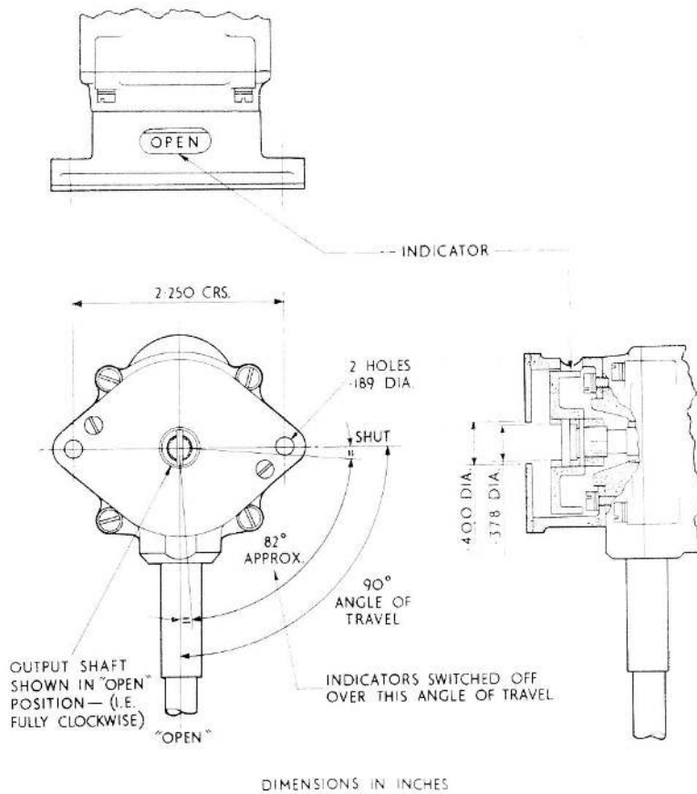
Fig. 2. Installation details
