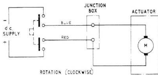
Fig. 1. Circuit diagram
