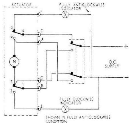
Fig. 1. Circuit diagram
