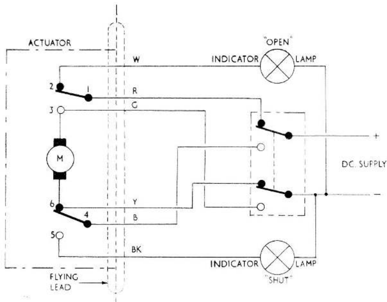
Fig. 1. Circuit diagram
