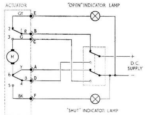
◀ Fig. 1. Circuit diagram ▶
