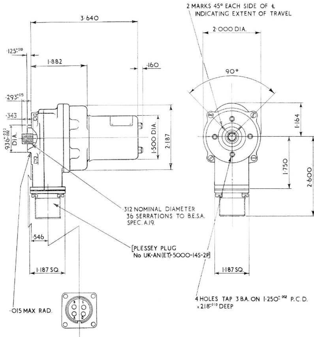
Fig. 2. Installation details
