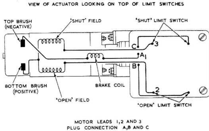
Fig. 4. Layout of internal wiring
