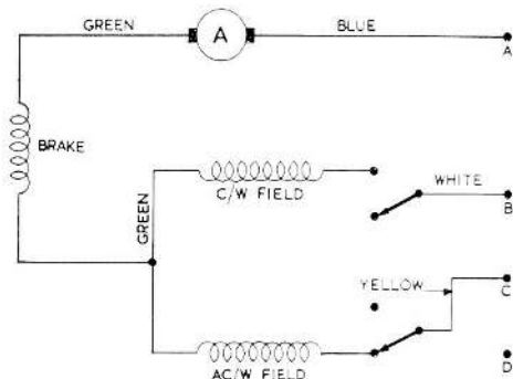
Fig. 3. Diagram of internal connections
