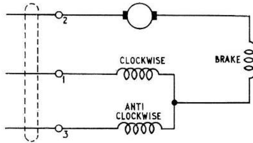
Fig. 2. Circuit diagram
