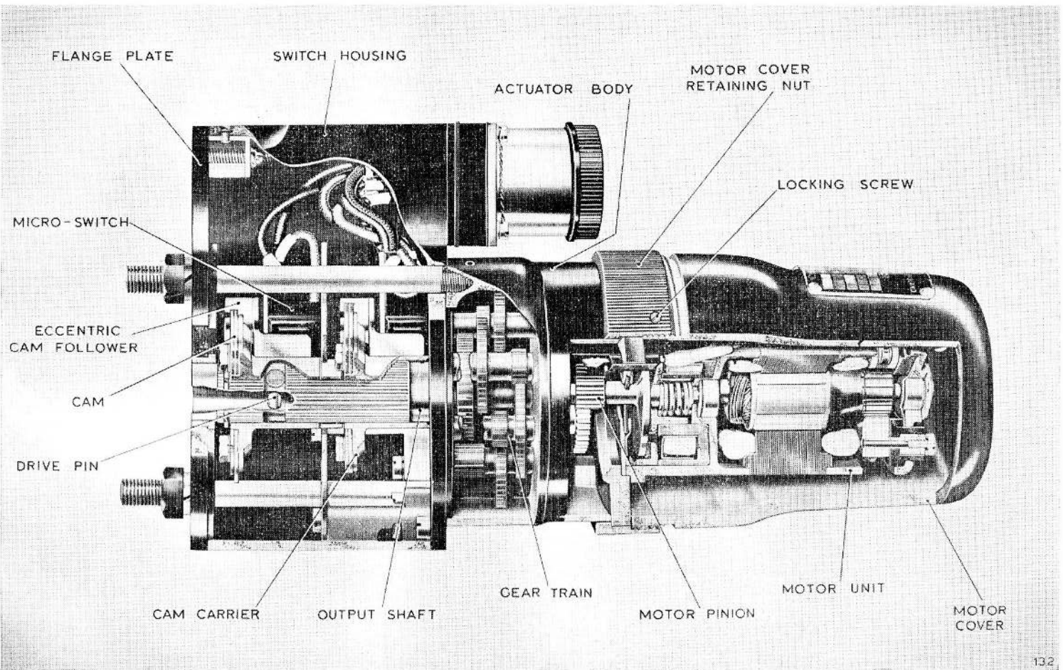
Fig. 1. Cut-away view of actuator RESTRICTED
