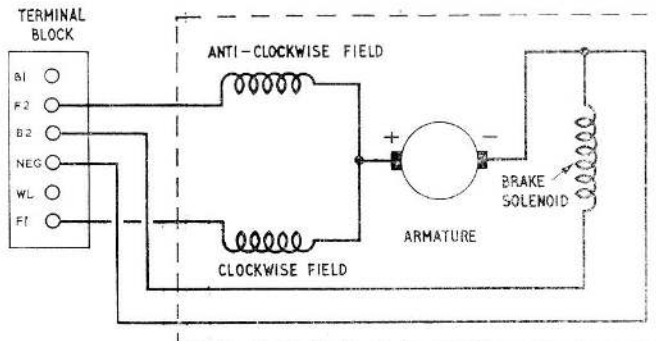
Fig. 2. Circuit diagram
