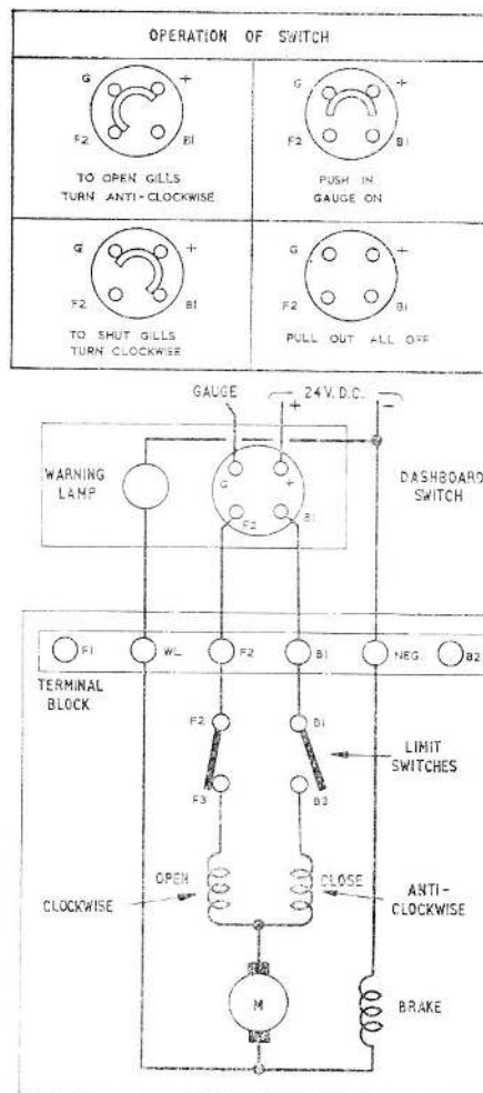
Fig. 3. Switch operation and wiring diagram
