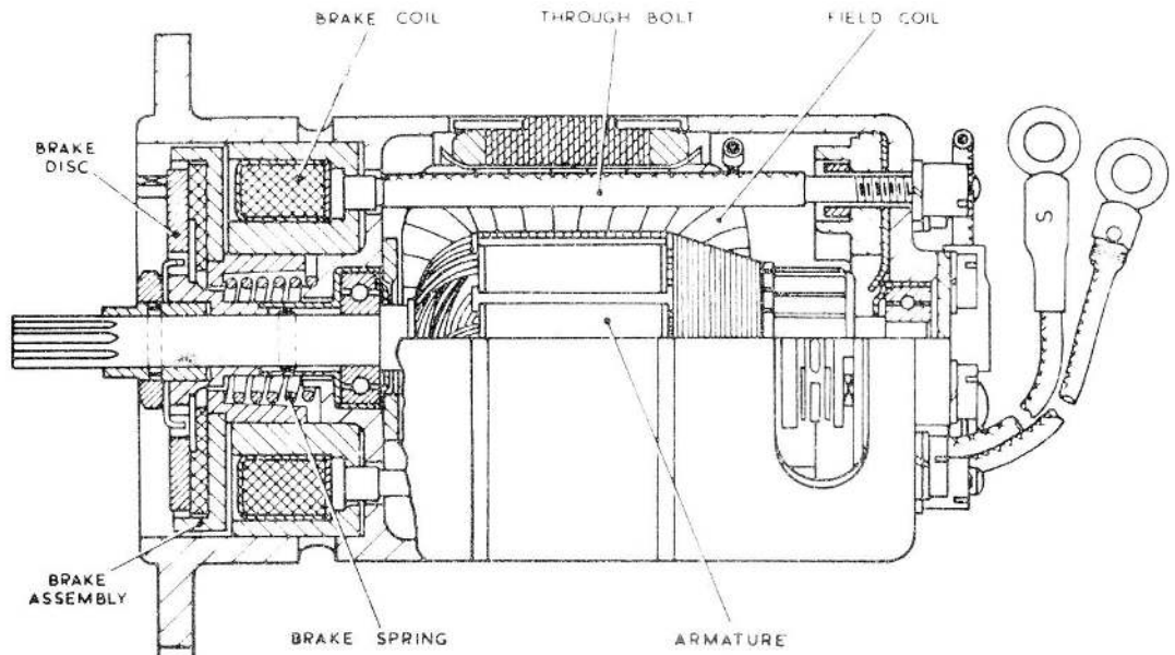
Fig.4. Sectional view of motor (Plessey type)
