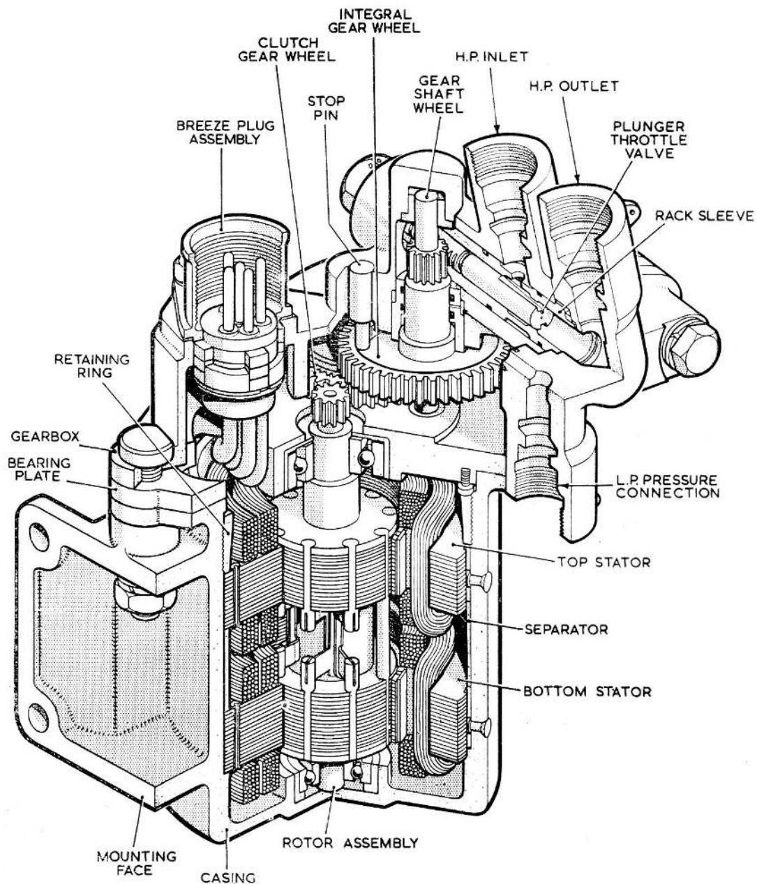
Fig. 1. Corrector unit, Type SNC/5
