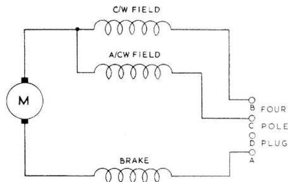
Fig. 2. Diagram of internal connections
