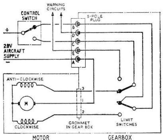
Fig. 4. Circuit diagram
