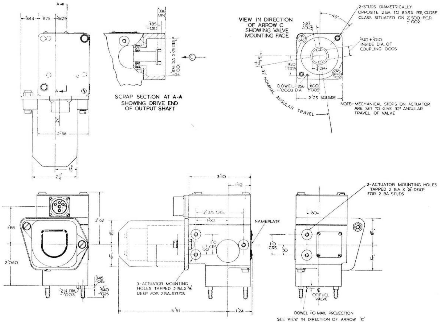
Fig. 5. Installation drawing
