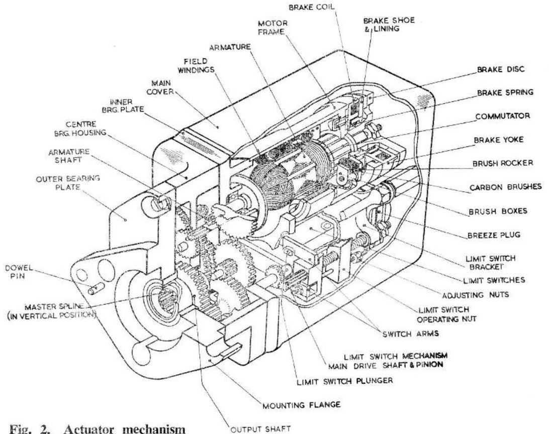
Fig. 2. Actuator mechanism
