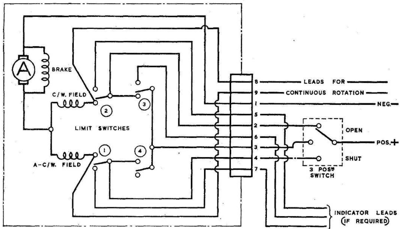
Fig. 3. Circuit diagram
