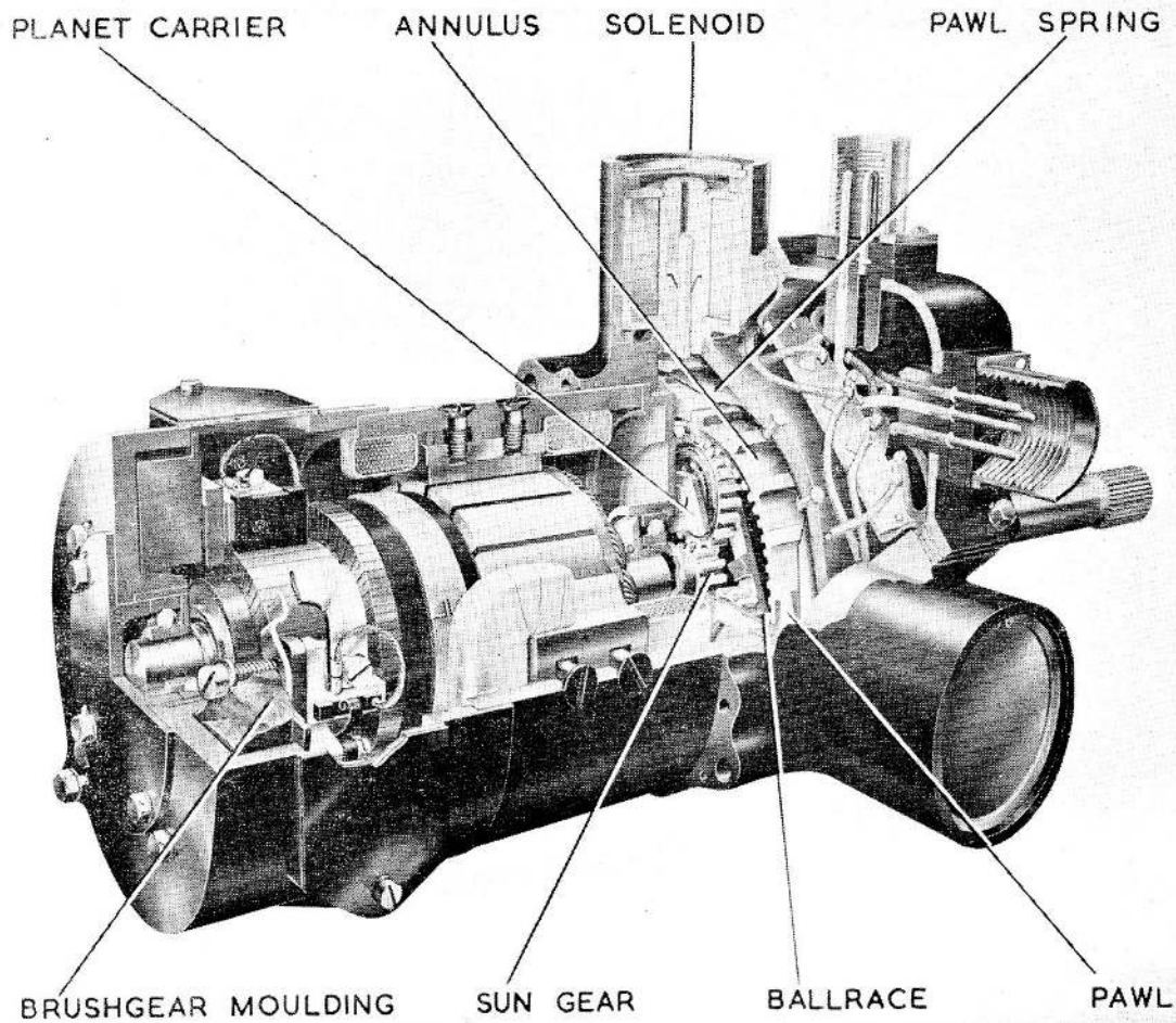
Fig. 1. Actuator, Rotax, Type C7001
