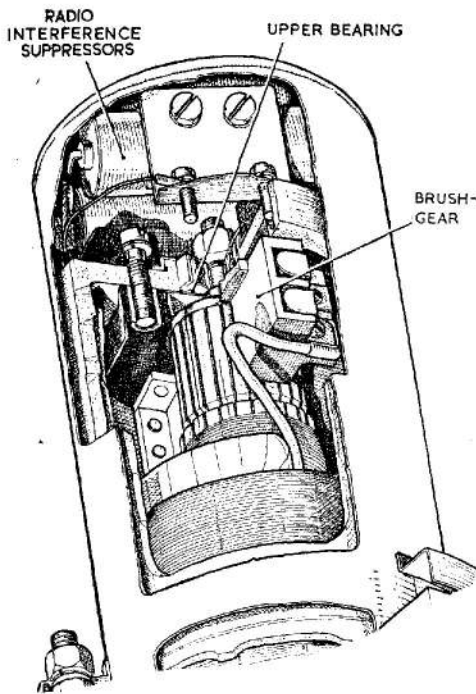
Fig. 3. Part sectional view of a typical B.P.1/RS fuel booster pump
