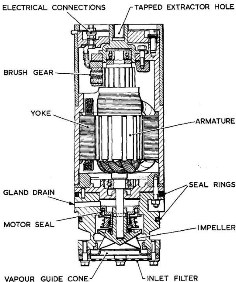
Fig. 4. Sectional view of type P.D.C.1001 Mk. 2 and Mk. 3 fuel pump
