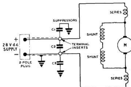
Fig. 1. Circuit diagram— B.P.14/RS, Mk. 2, 2A, 3 and 3A pumps
