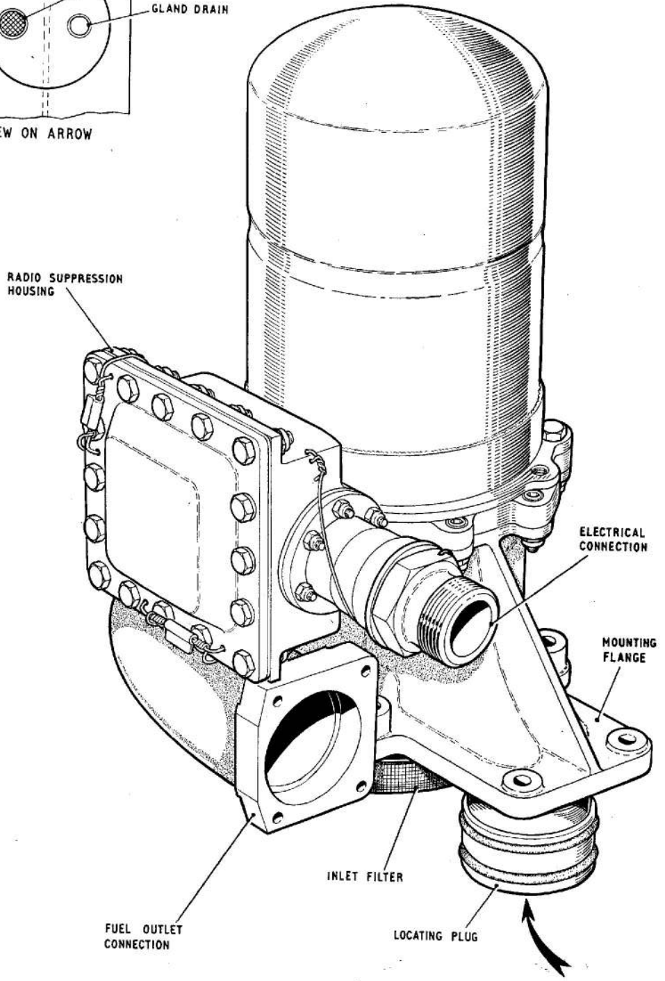
Fig. 1. General view of SPE.1302 pump
