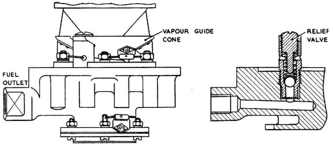
Fig. 2. Part sectional view of pump
