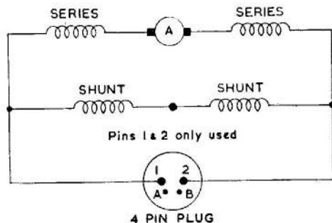
Fig. 6. Circuit diagram
