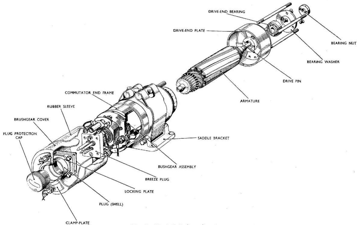
Fig. 7. Exploded view of motor
