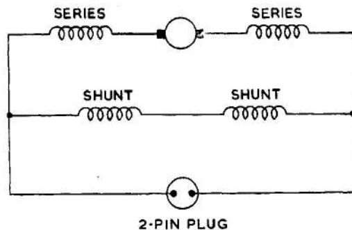
Fig. 4. Circuit diagram
