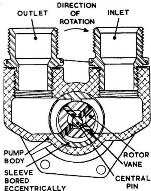
Fig. 3. Cross-sectional view
