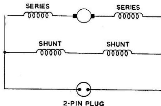
Fig. 4. Circuit diagram
