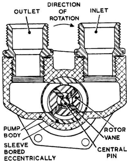
Fig. 3. Cross-sectional view
