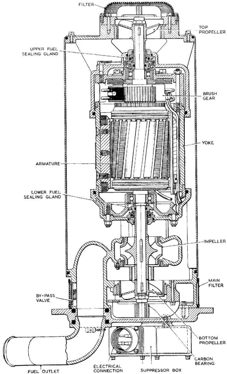
Fig. 2. Sectional view of PDC.2400 DE fuel pump
