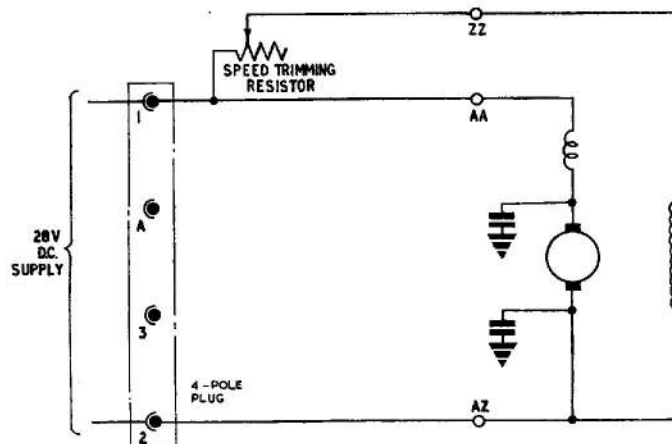
Fig. 4. Circuit diagram
