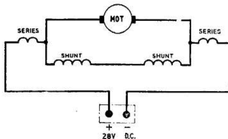
Fig. 4. Circuit diagram
