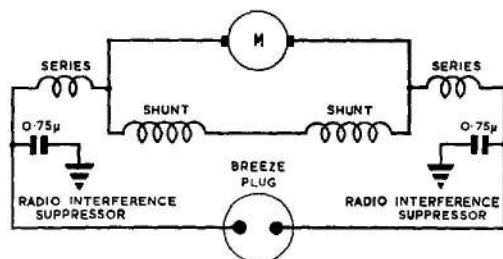
Fig. 3. Circuit diagram
