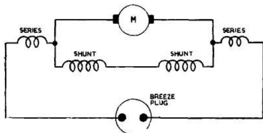
Fig. 3. Circuit diagram
