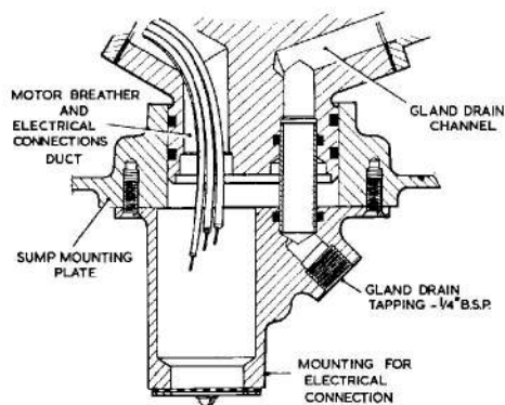
Fig. 3. Sectional view of SPE. 1236 gland drain
