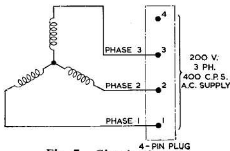
Fig. 7. Circuit diagram
