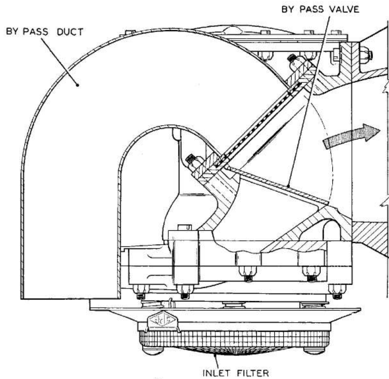
Fig. 2. Sectional view of SPE. 1234 Mk. 2 by-pass valve
