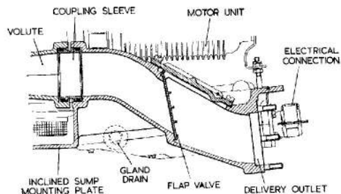
Fig. 3. Sectional view of outlet duct
