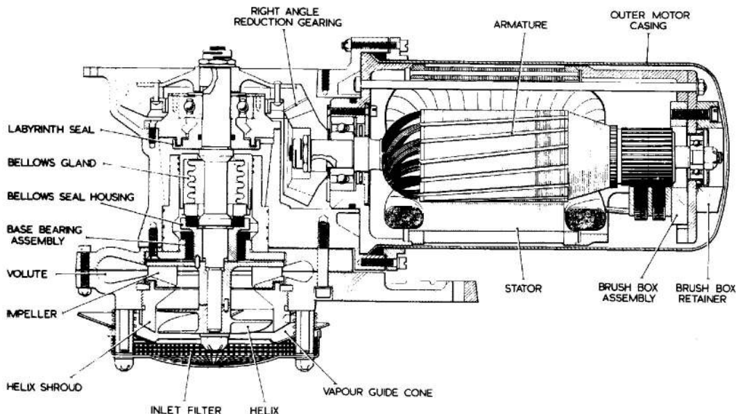
Fig. 2. Typical SPE.1200 series pump and motor unit assembly
