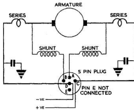
Fig. 3 Circuit diagram
