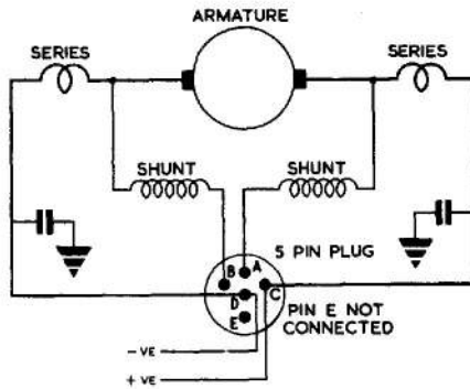
Fig. 3 Circuit diagram
