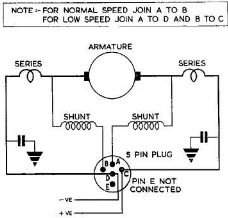
Fig. 3. Circuit diagram
