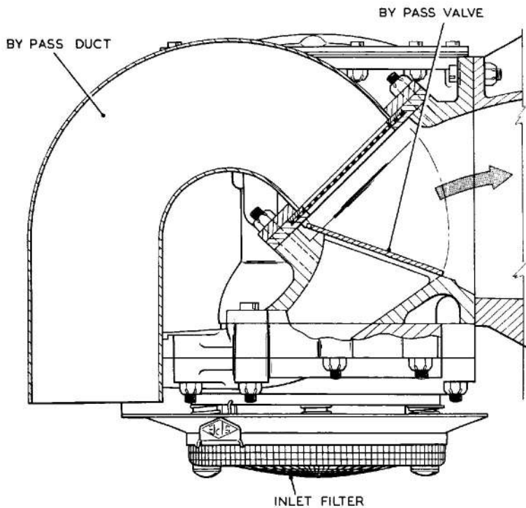
Fig. 2 Sectional view of SPE.1214 Mk.3 by-pass ducting
