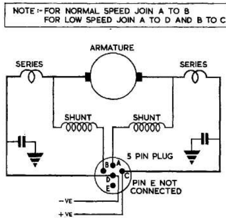
Fig. 3. Circuit diagram
