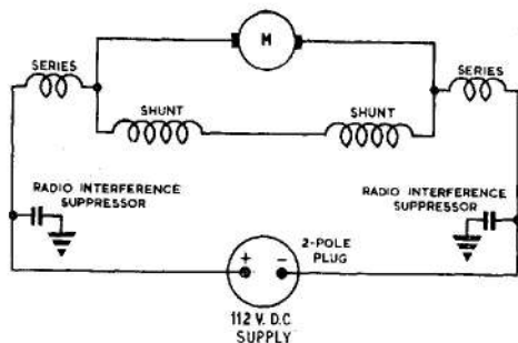
Fig. 4. Circuit diagram
