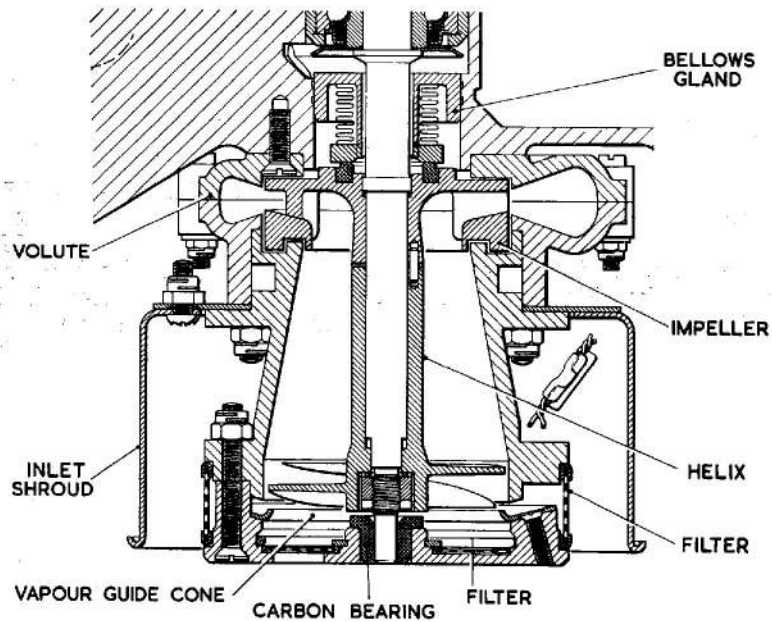
Fig. 1. Sectional view of SPE.404 Mk.IF pump unit
